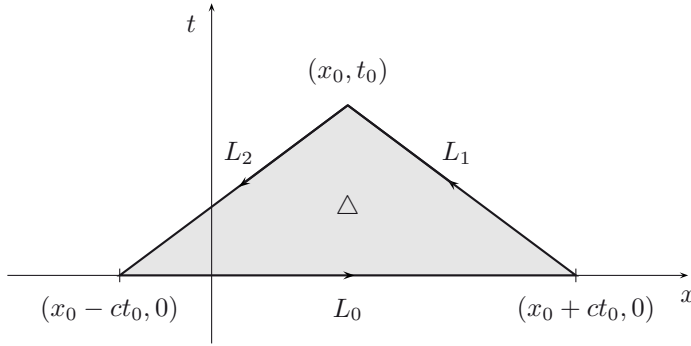
Figure 4.10 Characteristic triangle of the point (x_0, t_0) .
