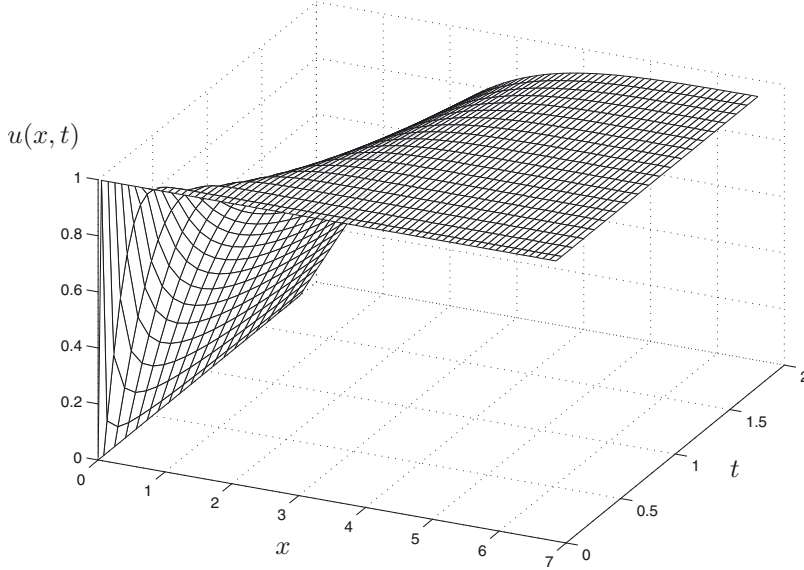
Figure 7.2 Solution of problem (7.5) with k = 1 .
