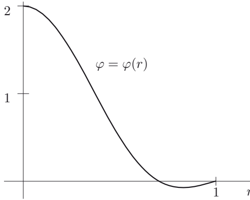
Figure 13.11 The initial displacement (13.44).
