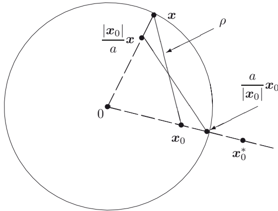
Figure 11.6 Congruent triangles and the proportionality of \rho and \rho^* .
