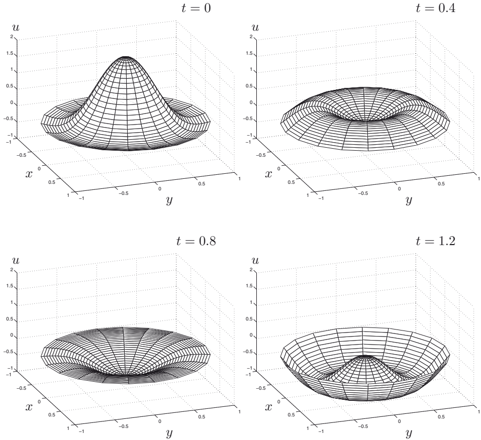
Figure 13.8 Solution of the initial boundary value problem (13.29) with initial condition (13.31) on time levels t = 0, 0.4, 0.8, 1.2 .
