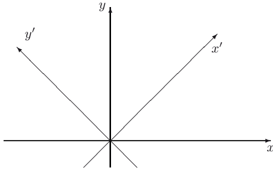
Figure 3.6 Transformation of the coordinate system.
