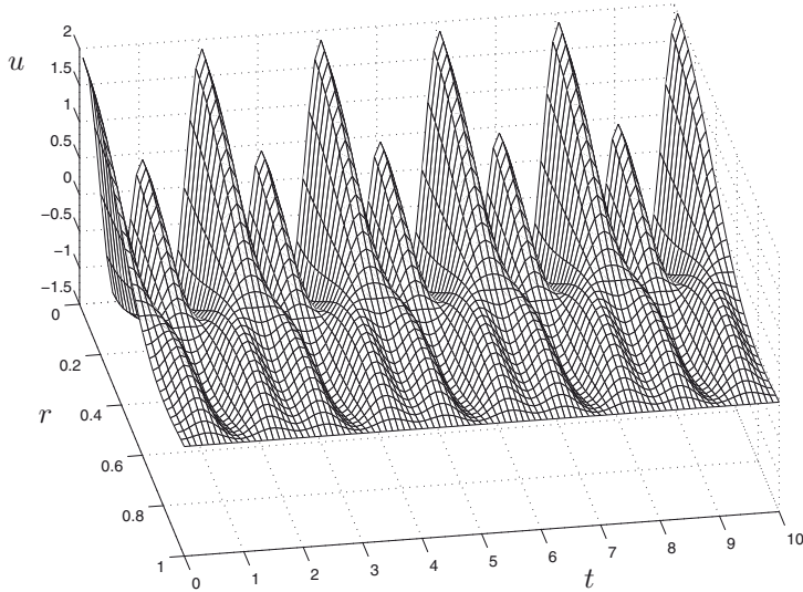
Figure 13.10 Solution of the initial boundary value problem (13.41) with initial condition (13.44).
