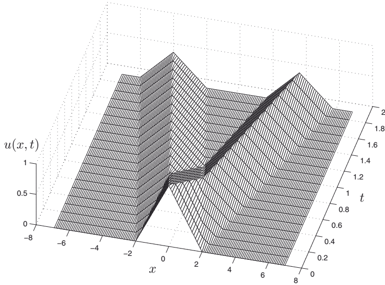
Figure 4.4 Graph of solution from Example 4.4 for c = 2 , b = 1 , a = 2 .
