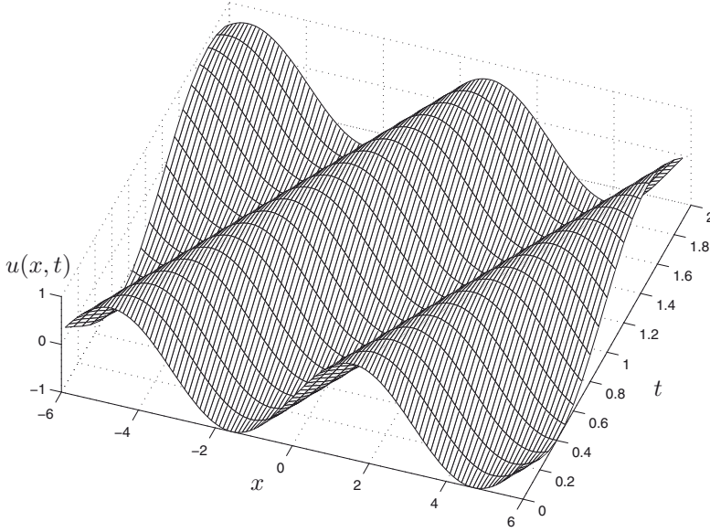
Figure 3.5 Solution of u_t + 3u_x = 0 , u(x, 0) = \sin x .
