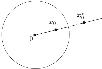
Figure 11.5 Ball \Omega and spherical inversion.
