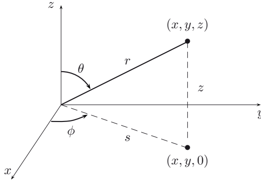
Figure 11.1 Spherical coordinates.
