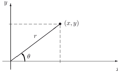
Figure 6.1 Polar coordinates r and \theta .
