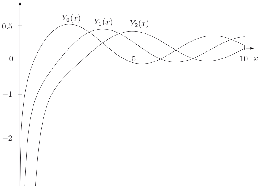
Figure 14.2 Bessel functions of the second kind for n = 0, 1, 2 .
