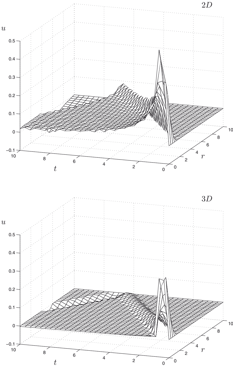
Figure 13.12 Radially symmetric solutions of the Dirichlet problem for the wave equation in 2D and 3D with the initial condition \psi(r) = 1 for 0 \leq r \leq 1 and zero otherwise.
