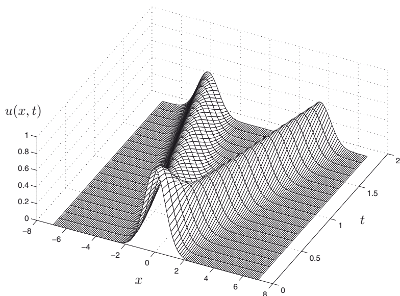
Figure 4.11 Solution of problem (4.26).
