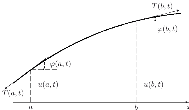
Figure 4.1 String segment.
