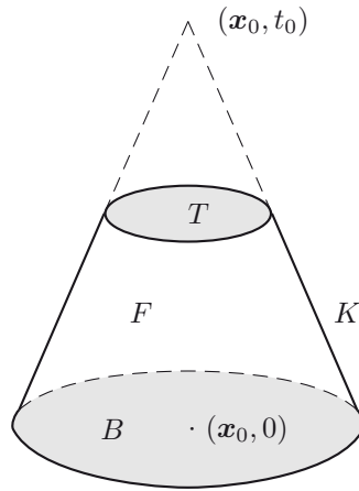
Figure 13.4 Solid cone frustum F .
