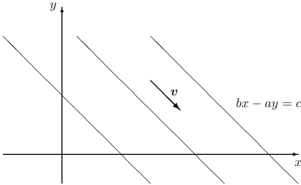
Figure 3.2 Characteristic lines.
