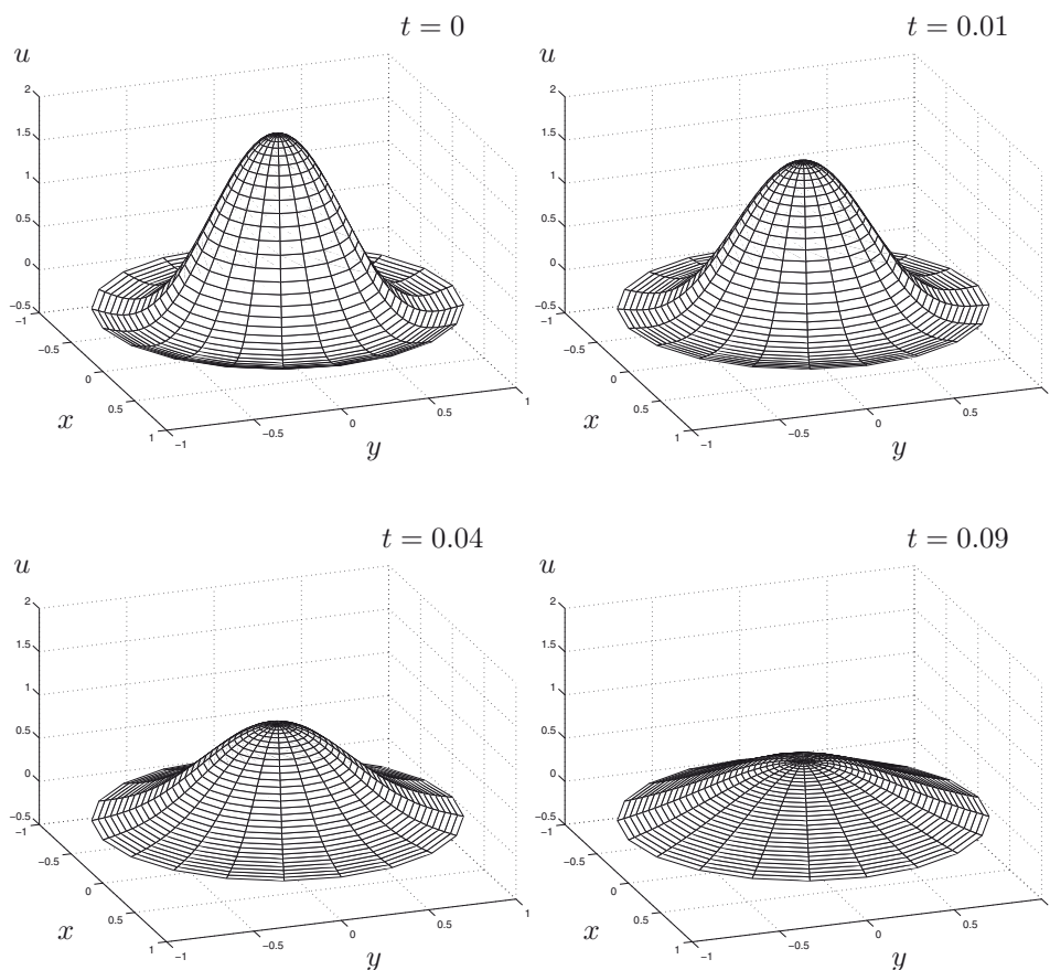
Figure 12.3 Solution of the initial boundary value problem (12.17) with initial condition (12.18) on time levels t = 0, 0.01, 0.04, 0.09 .
