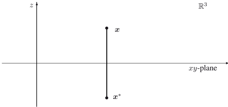
Figure 11.3 Half-space and reflection method.
