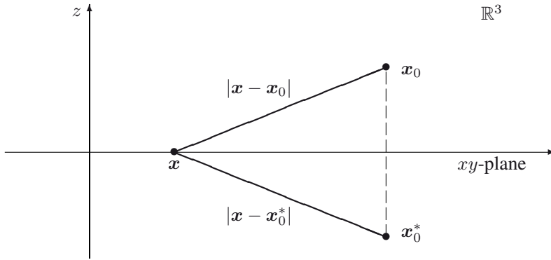
Figure 11.4 Verification of the property (ii) of Green's function.
