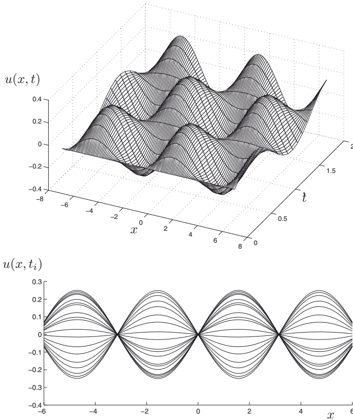
Figure 4.2 Standing waves—a solution of the initial value problem (4.16) with c = 4 .
