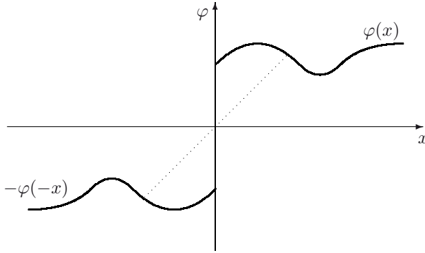
Figure 7.1 The odd extension.
