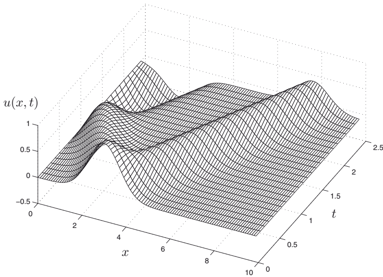
Figure 7.4 Solution of problem (7.10) for c = 2 .
