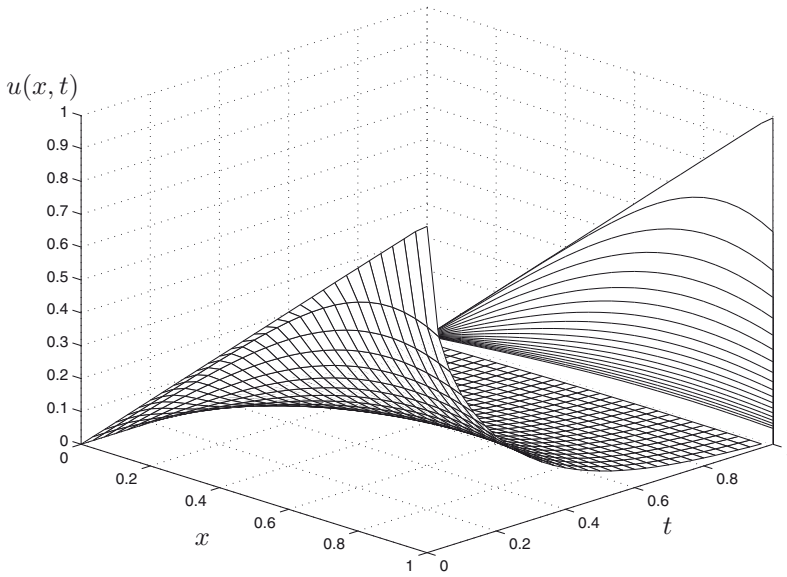
Figure 7.12 Graphic illustration of the solution u(x, t) of problem (7.41) for h = 1 , k = 1 .
