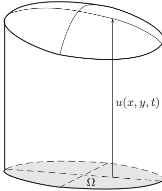
Figure 13.1 Vibrating membrane over the subdomain \Omega .
