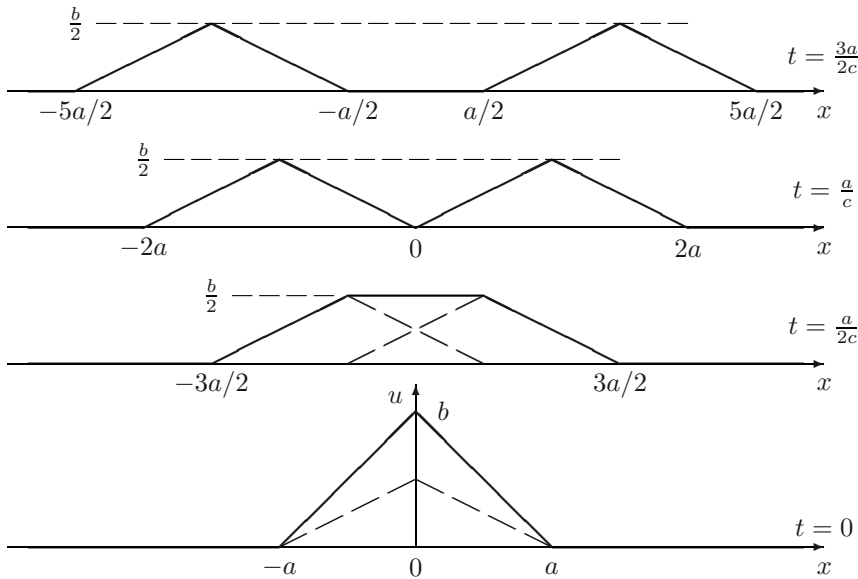
Figure 4.3 Solution of Example 4.4 on particular time levels.
