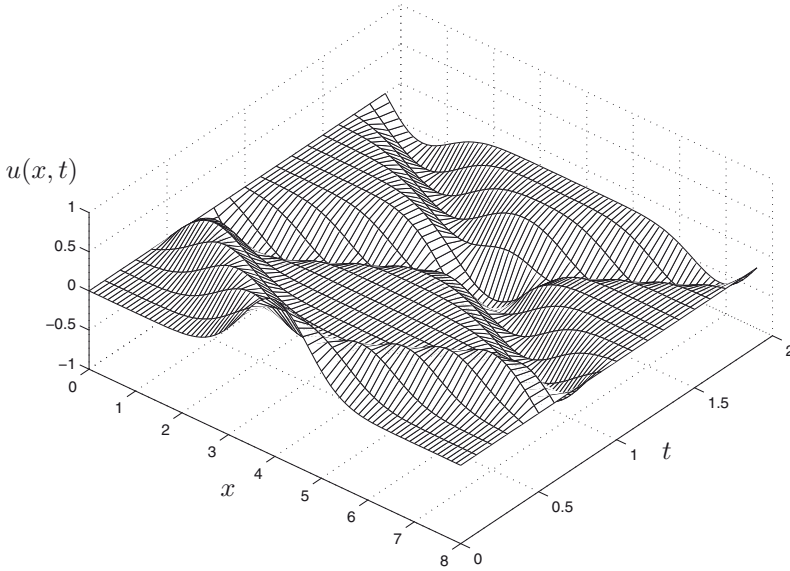
Figure 7.7 Solution of problem (7.26).
