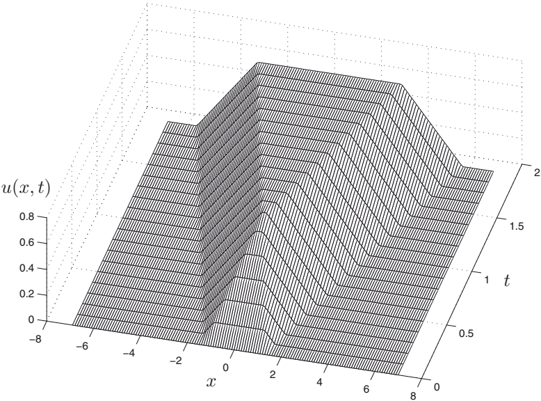
Figure 4.6 Graph of solution from Example 4.5 for c = 2.3 , a = 1.3 .
