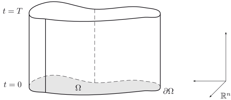
Figure 12.4 Space-time cylinder \Omega \times [0, T] .
