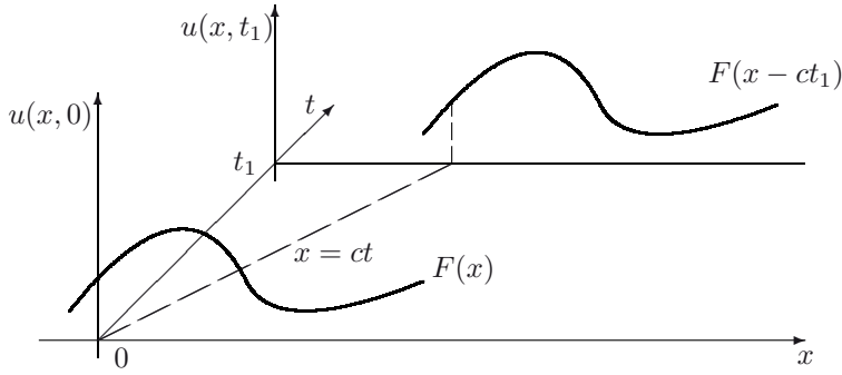
Figure 3.1 Traveling wave.
