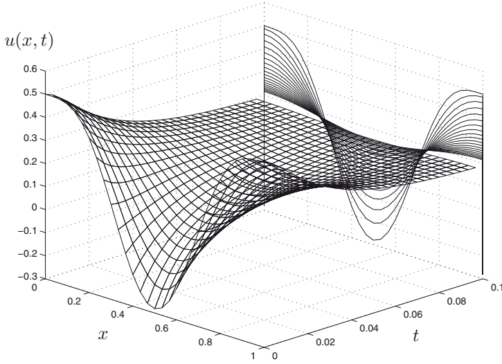
Figure 7.9 Solution of problem (7.40).
