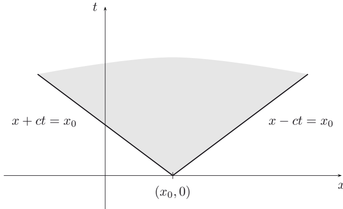
Figure 4.7 Domain of influence of the point (x_0, 0) at time t \geq 0 .
