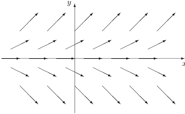
Figure 3.7 Vector field v = (1, y) .
