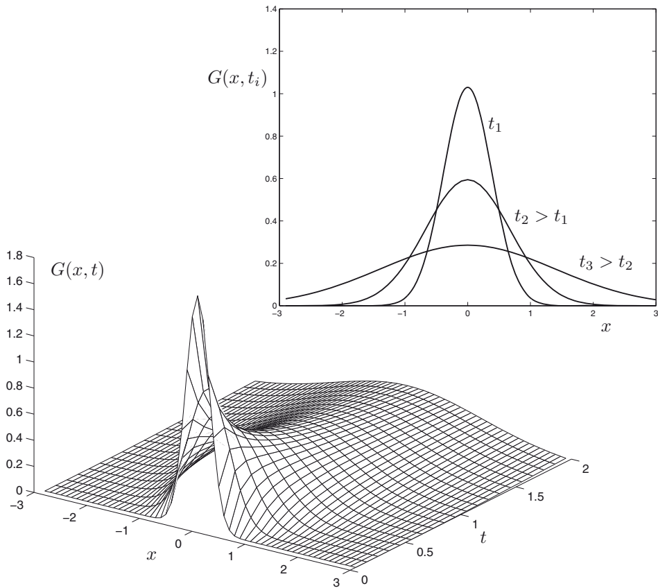
Figure 5.2 Fundamental solution of the diffusion equation (here, with the choice k = 0.5 ).
