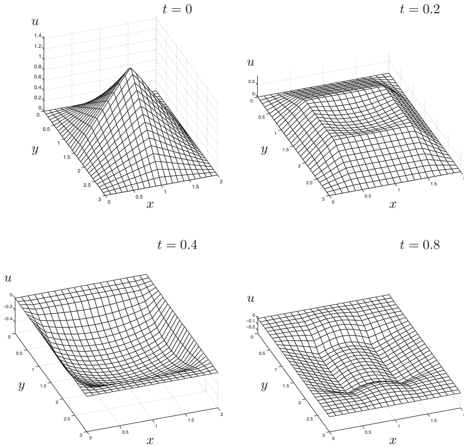
Figure 13.6 Solution of the initial boundary value problem (13.24) for the data c = 3 , a = 2 , b = 3 , on time levels t = 0, 0.2, 0.4, 0.8 .
