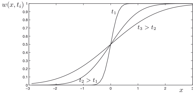
Figure 5.1 Temperature profile on several time levels for a step initial temperature.
