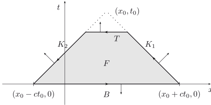
Figure 10.2 Trapezoid of characteristic triangle.
