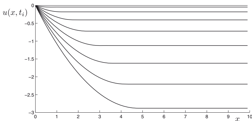
Figure 9.1 A string falling due to the gravitation.
