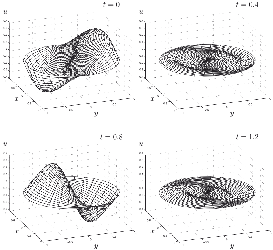
Figure 13.9 Solution of the initial boundary value problem (13.32) with initial condition (13.35) on time levels t = 0, 0.4, 0.8, 1.2 .
