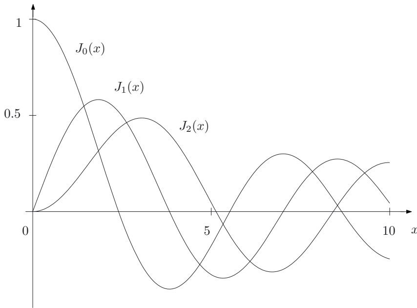
Figure 14.1 Bessel functions of the first kind for n = 0, 1, 2 .
