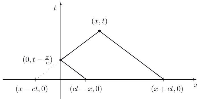
Figure 7.3 Reflection method for the wave equation.
