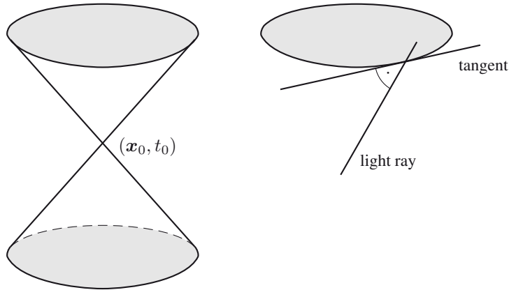
Figure 13.3 Light cone at a point (\mathbf{x}_0, t_0) , \mathbf{x}_0 \in \mathbb{R}^2 , and orthogonality of light rays to the sphere |\mathbf{x} - \mathbf{x}_0| = c|t - t_0| .
