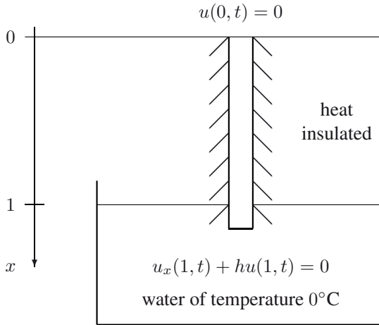
Figure 7.10 Schematic illustration of problem (7.41).
