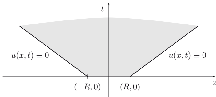
Figure 4.8 Domain of influence of the interval (-R, R) at time t \geq 0 .
