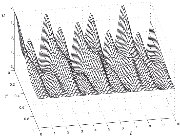
Figure 13.7 Solution of the initial boundary value problem (13.29) with initial condition (13.31)—dependence on r and t .
