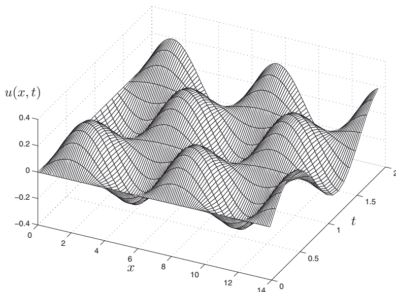
Figure 7.5 Solution of problem (7.11) for c = 4 .
