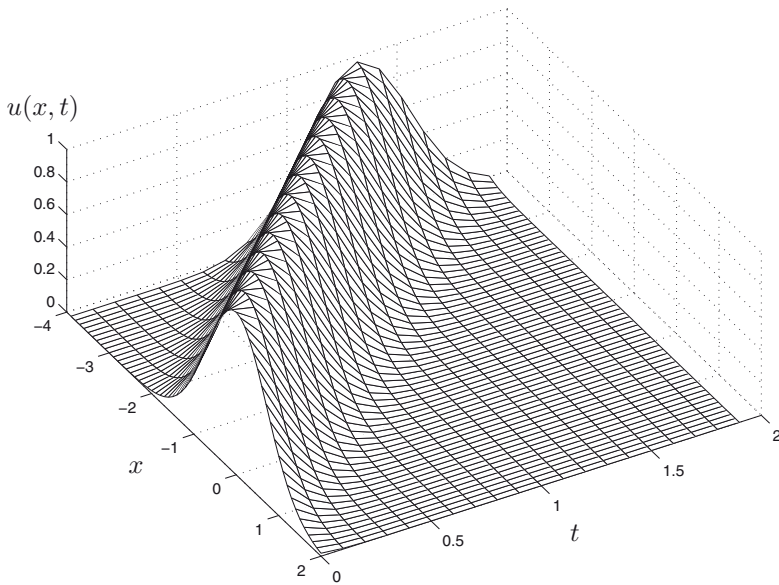
Figure 3.4 Solution of u_t - 3u_x = 0 , u(x, 0) = e^{-x^2} .
