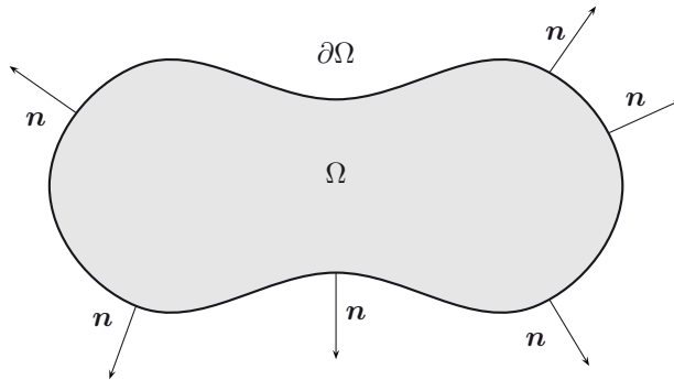
Figure 11.2 Domain \Omega with the unit vector of the outer normal to the boundary.
