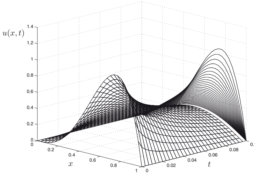
Figure 7.8 Solution of problem (7.36).
