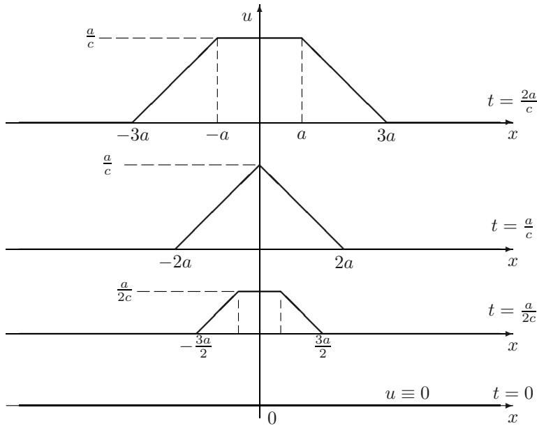
Figure 4.5 Solution of Example 4.5 on particular time levels.
