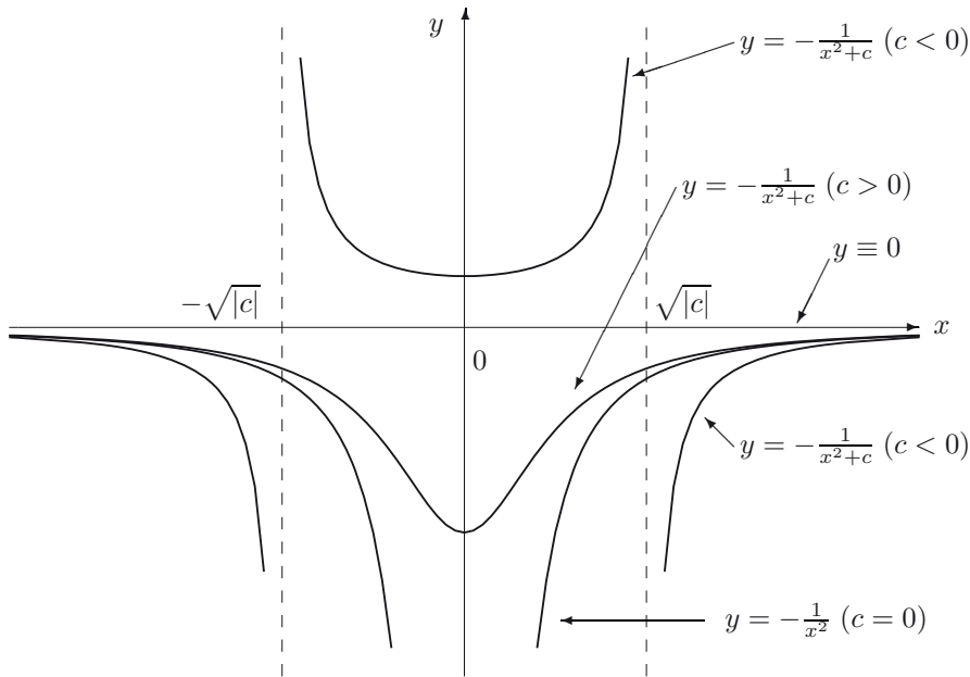
Figure 3.8 Characteristics of the equation u_x + 2xy^2u_y = 0 .
