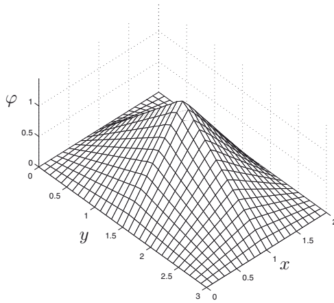
Figure 13.5 Initial condition (13.25) with the choice a = 2 , b = 3 .
