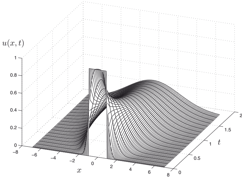
Figure 5.3 Solution of Example 5.4 with k = 2 .
