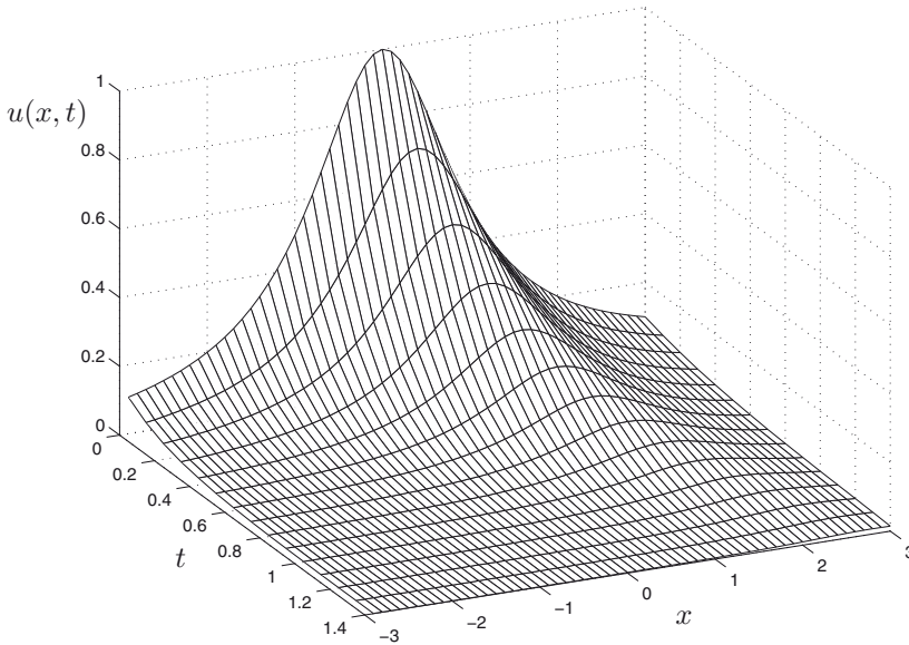
Figure 3.9 Solution of the problem u_t + 2u_x = -3u , u(x, 0) = 1/(1+x^2) .
