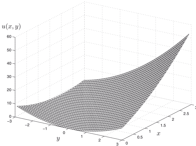
Figure 3.3 The solution from Example 3.1.
