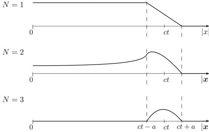
Figure 13.2 “Hammer blow” in one, two and three dimensions.
