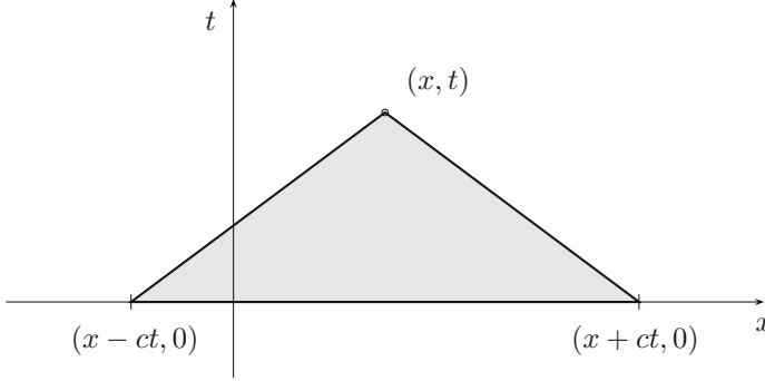
Figure 4.9 Domain of dependence of the point (x, t) .
