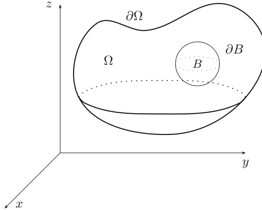
Figure 12.1 An arbitrary closed ball B in a domain \Omega .
